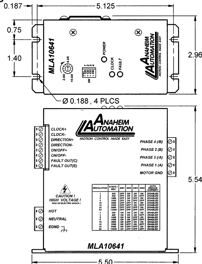
Figure 1: MLA10641 Dimensions
